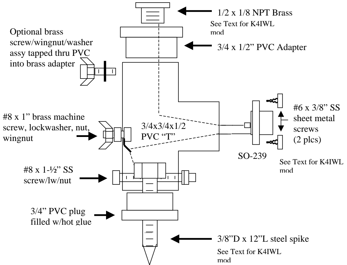
Figure 4 – Base Assembly
