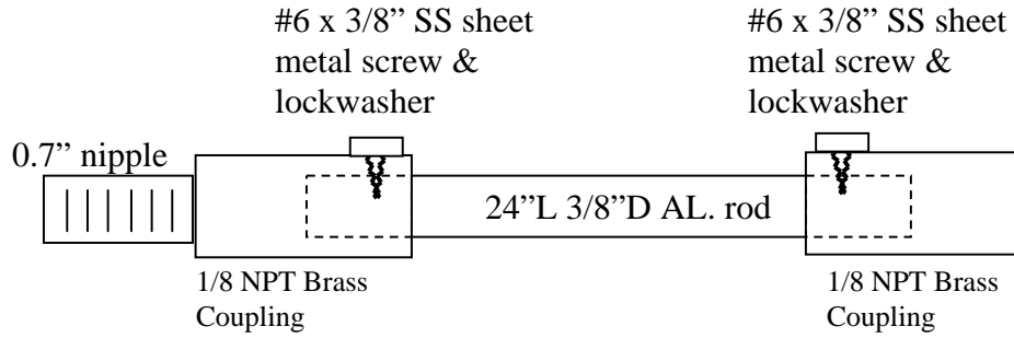
Figure 1 - Middle Sections, no coil (3 ea)
