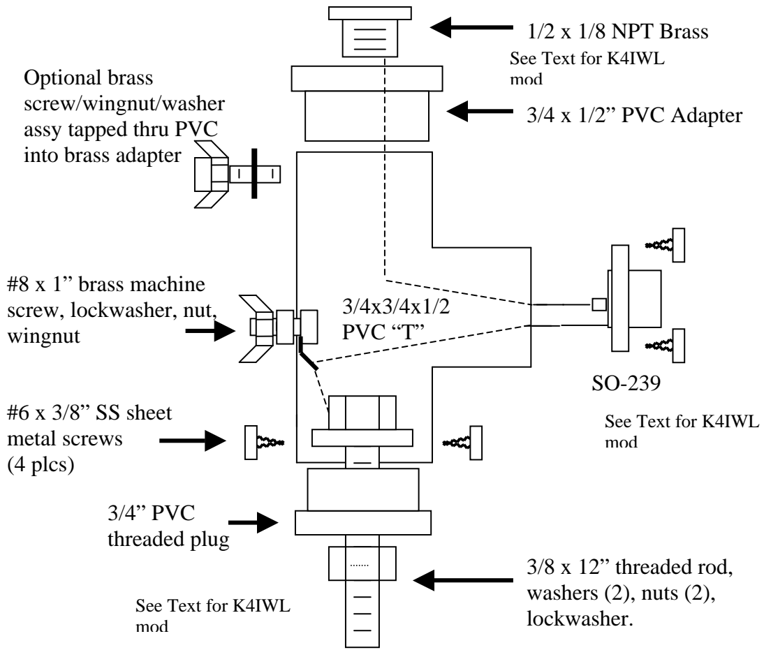
Figure 7 – Optional Base Assembly
