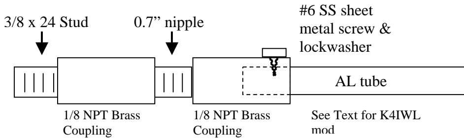
Figure 5 – Adapt to Standard 3/8x24 base
