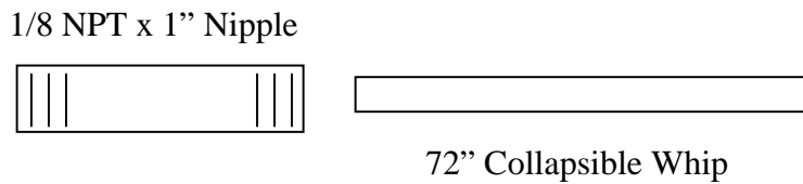
Figure 3 – Collapsible whip assembly
