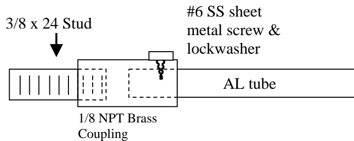
Figure 6 – Alternate Adapt to Standard 3/8x24 base
